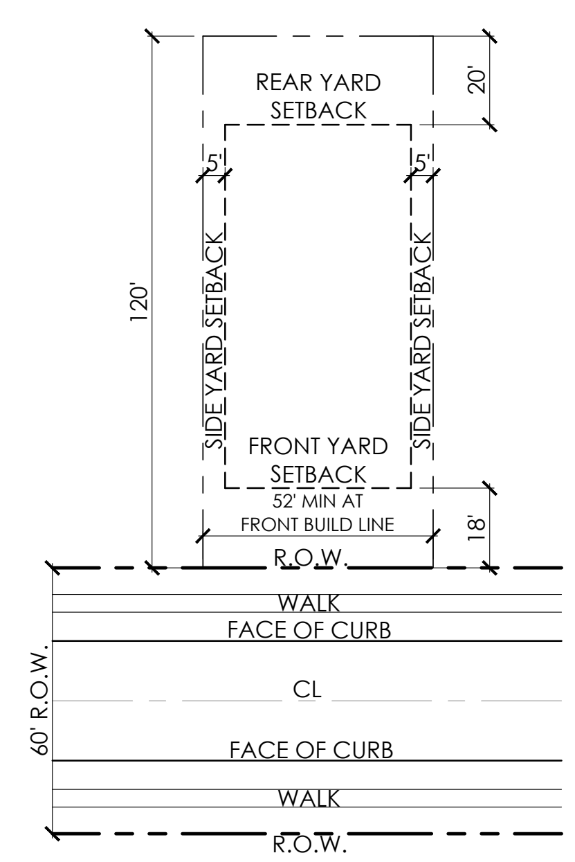
1 TYP. 52' x 120' LOT CONFIGURATION SCALE: 1" = 30'
