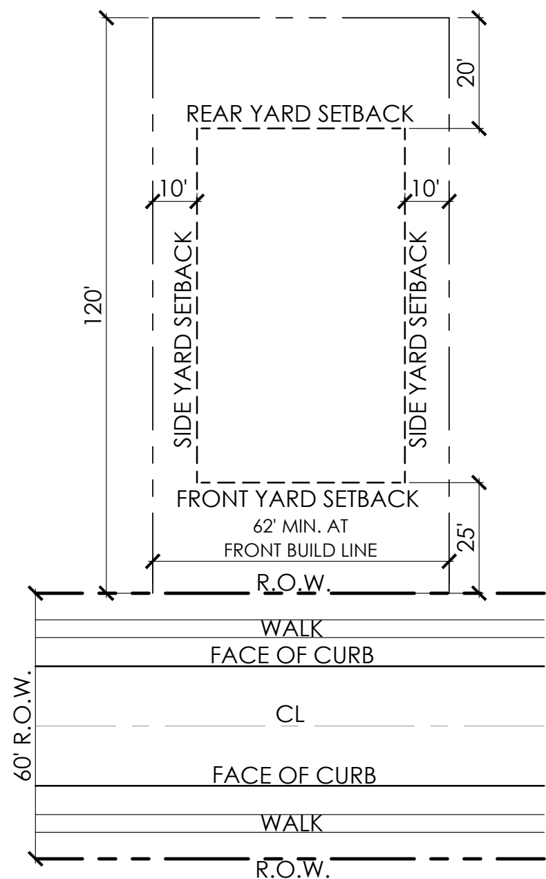
① TYP. 62' X 120' LOT CONFIGURATION SCALE: 1" = 30'
