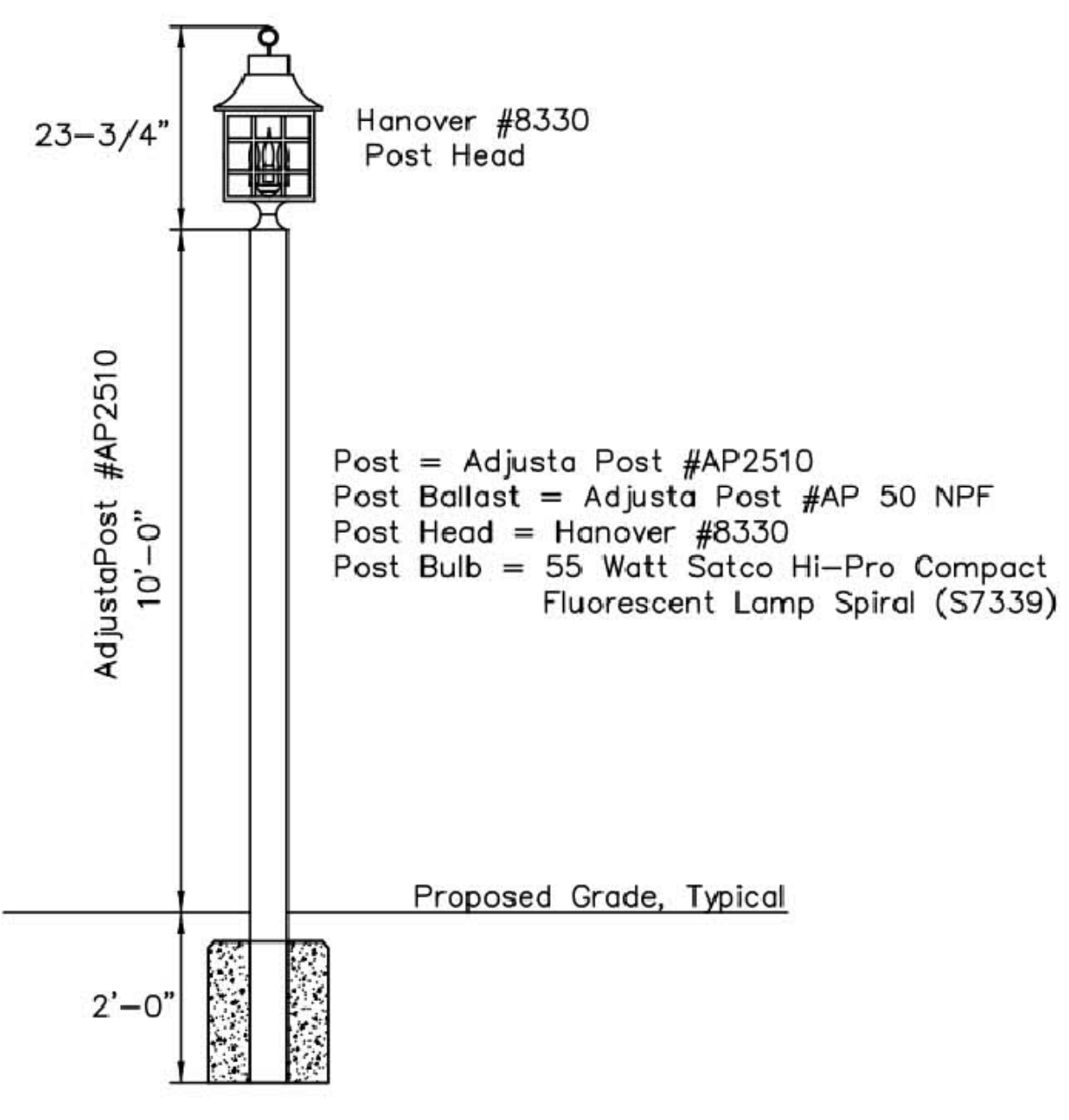
STANDARD LIGHT POLE Not to Scale
