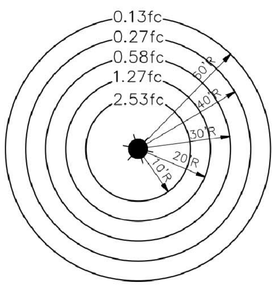
TYPICAL LIGHT POLE PHOTOMETRICS Not to Scale
